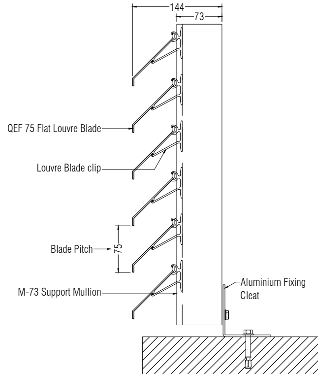
Section of Blades & Mullion
