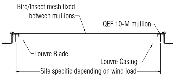
Plan Detail
