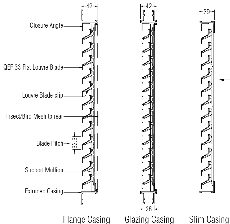
Section with Mullion & Casing
