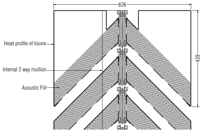
QEF AC300 D/B Louvre Head Detail
