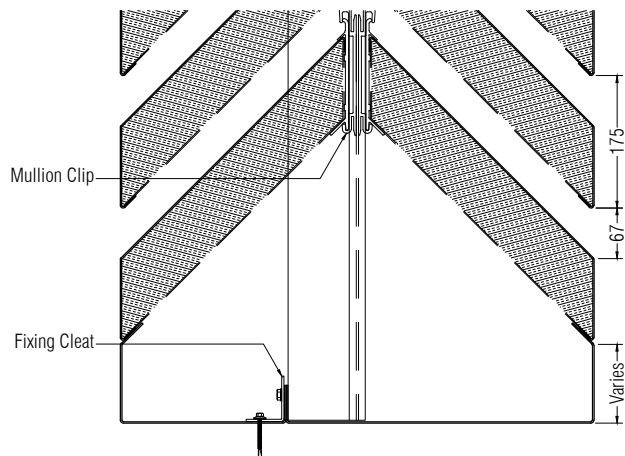
QEF AC300 D/B Louvre Base Details
