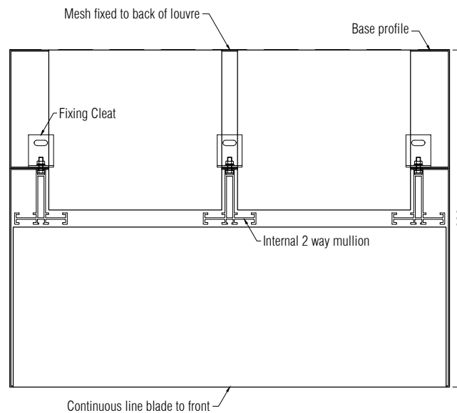
QEF AC300 D/B Louvre Plan view
