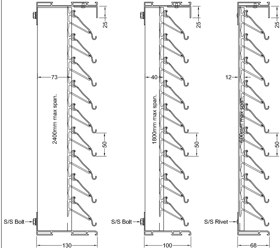
QEF 50HP Profile Louvre with Long Span Mullion
