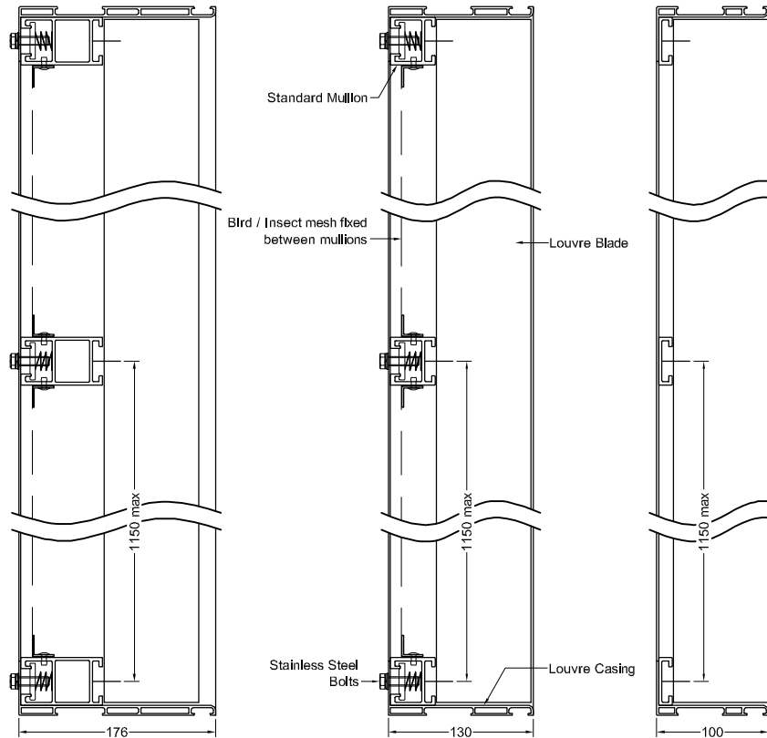
QEF 50 Chevron Louvre with Long Span Mullion
