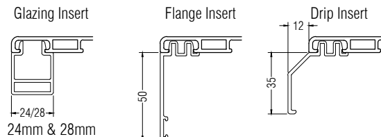
Casing Insert Options
