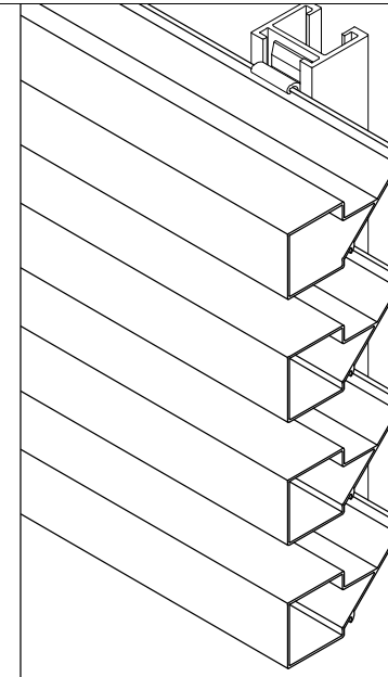
Isometric Detail
