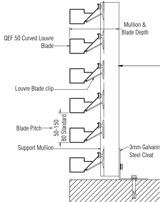
Section with Mullion & Casing
