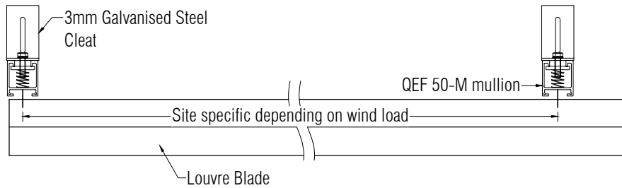
Plan Detail
