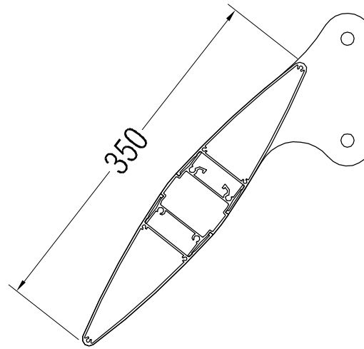
STRUCTURAL END PLATE DETAIL
