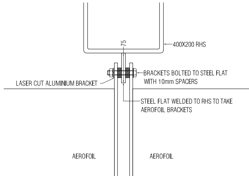
STRUCTURAL END PLATE DETAIL
