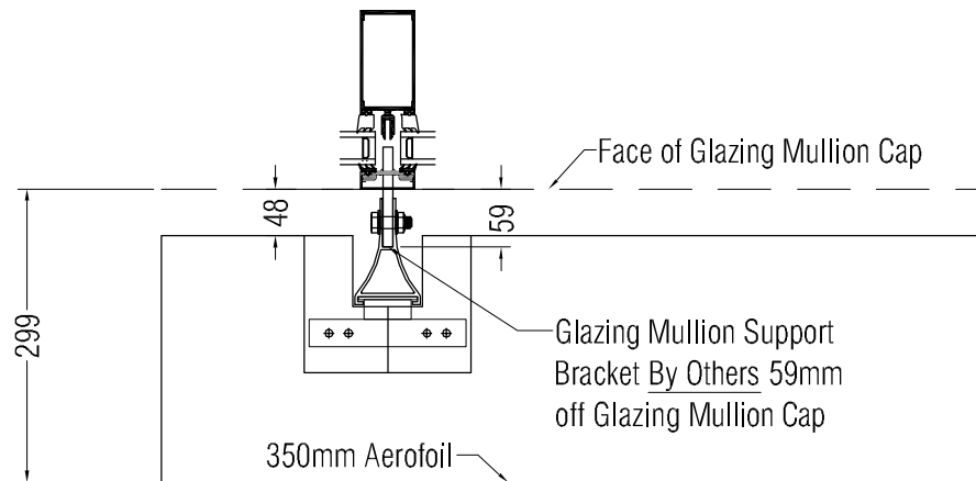
PLAN DETAIL OF AEROFOIL CONNECTION
