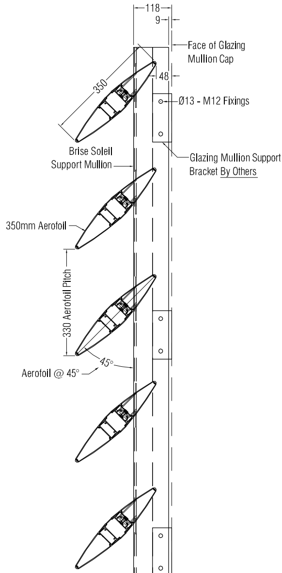
TYPICAL SECTION DETAILS
