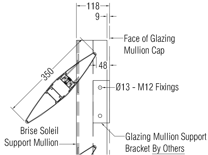
AEROFOIL MULLION CONNECTION
