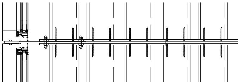
CEDAR PLANK FIXING DETAILS
