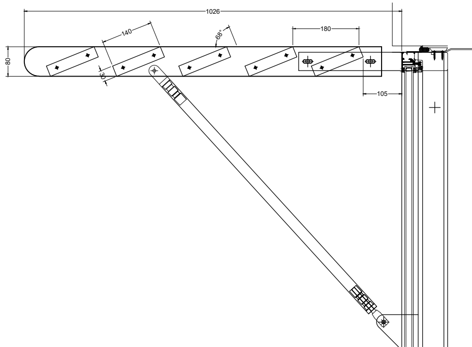
SIDE VIEW WITH STRUT
