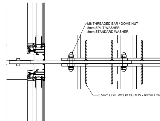
BRACKET FIXING DETAILS
