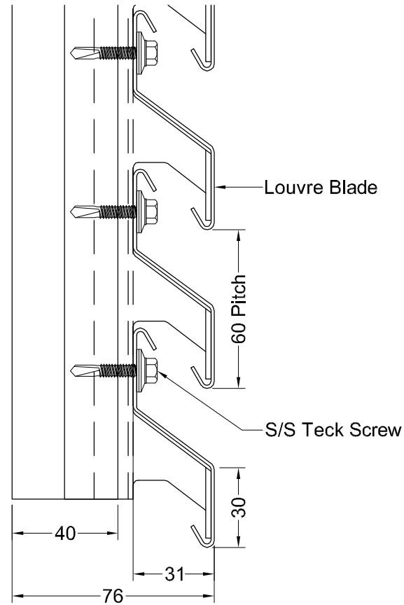
QEF - Galv Louvre Fixed Details
