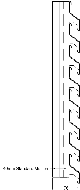
QEF - Galv Louvre Fixed to Standard Mullion
