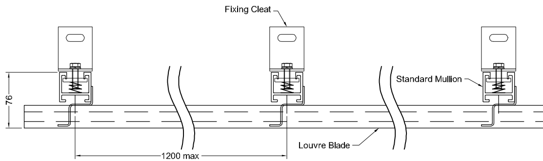
QEF - Galv Louvre Plan Fixed to Standard Mullion
