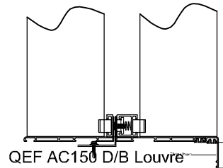
QEF AC150 D/B Louvre Head Detail
