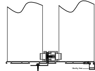
QEF AC150 D/B Louvre inserts
