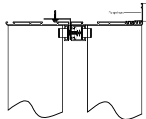
QEF AC150 D/B Louvre Head Detail
