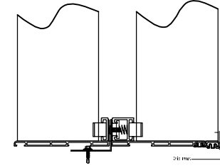
QEF AC150 D/B Louvre Section Details
