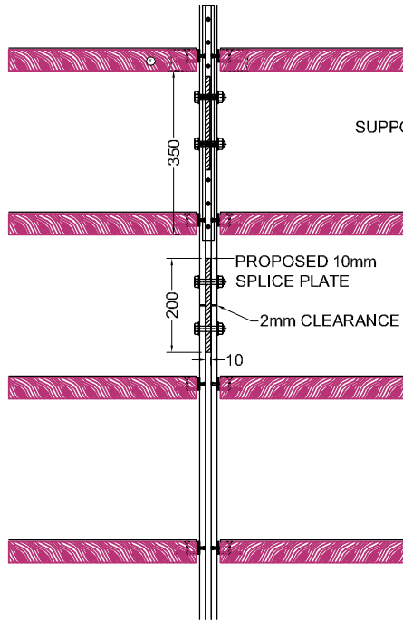
FRONT & SIDE VIEWS
