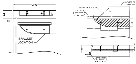
4.8 mm SLOT DETAIL AND SCREW HOLE DETAILS
