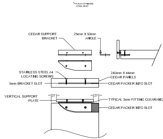
FRONT & SIDE VIEWS
