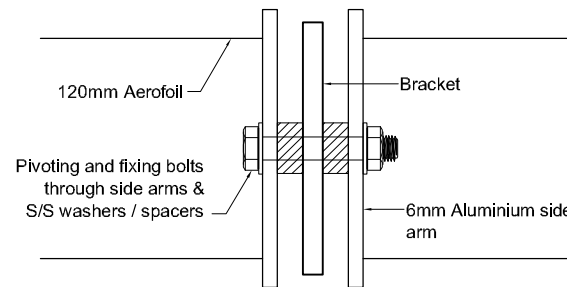
END SECTION THROUGH MODULE JOINT SHOWING BOLT
