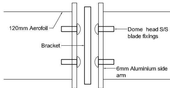
END SECTION THROUGH MODULE JOINT SHOWING BUTTON HEAD AEROFOIL FIXINGS
