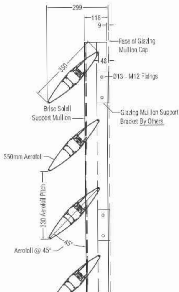
350 Aerofoil Fixing Details Scale 1:10
